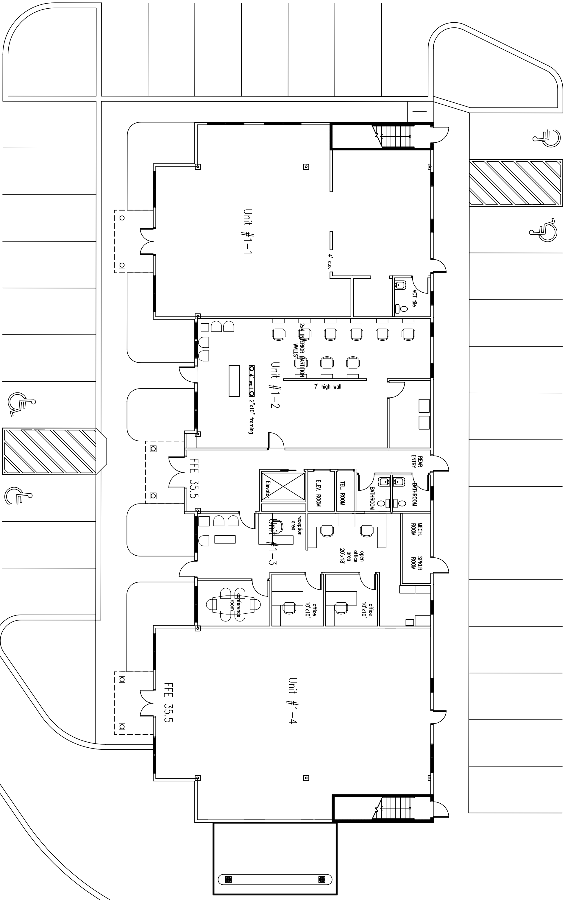
York Village Business Center FIRST FLOOR LAYOUT
